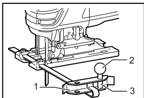
1. Fence guide 2. Threaded knob 3. Circular guide pin
