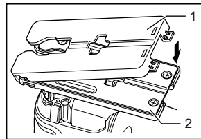
1. Cover plate 2. Base
